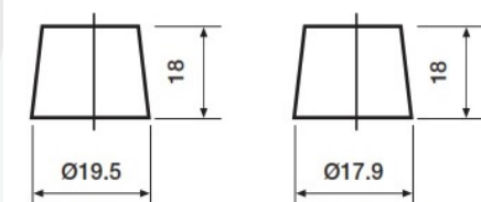
Positive Terminal
